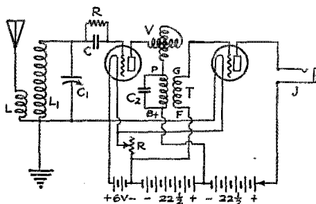
THE CIRCUIT
