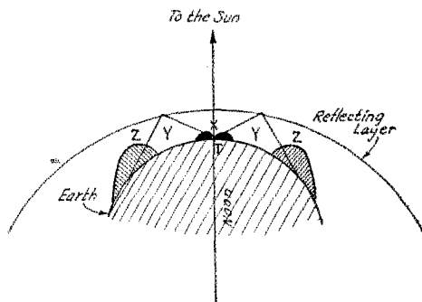
FIG. 4 THE NATURE OF "SKIPPED DISTANCE" OR "DEAD BELT."
