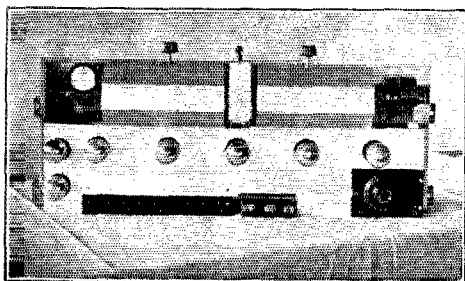
FIG. 3 TOP VIEW OF THE SET.
