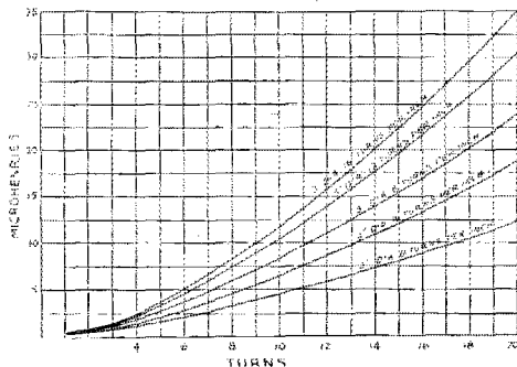
THE INDUCTANCE CHART
